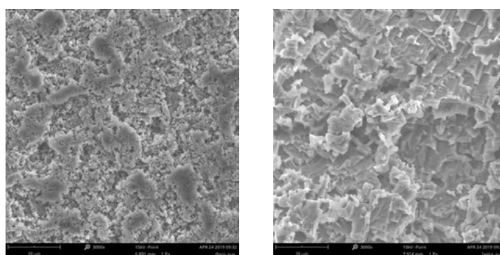
Fig.1 - a) Structure of the etched aluminium plate in: a) lab scale; b) towing tank scale.
