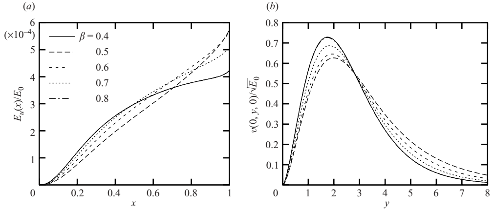
FIGURE 17. Comparison at fixed control energy E_w = 1 for increasing wavenumber \beta , E_0 = 1 : (a) perturbation energy E_u(x)/E_0 ; (b) optimal perturbation v_0(x, y, 0)/\sqrt{E_0} in the plane z = 0 .
