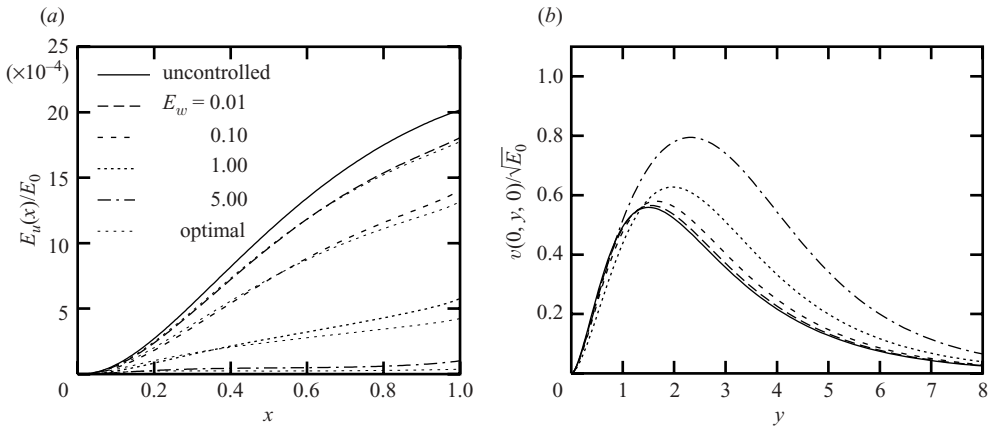
FIGURE 15. Comparison at constant wavenumber \beta = 0.547 for increasing control energy E_w at E_0 = 1 : (a) perturbation energy E_d(x)/E_0 ; (b) optimal perturbation v_0(y, z)/\sqrt{E_0} in the plane z = 0 .
