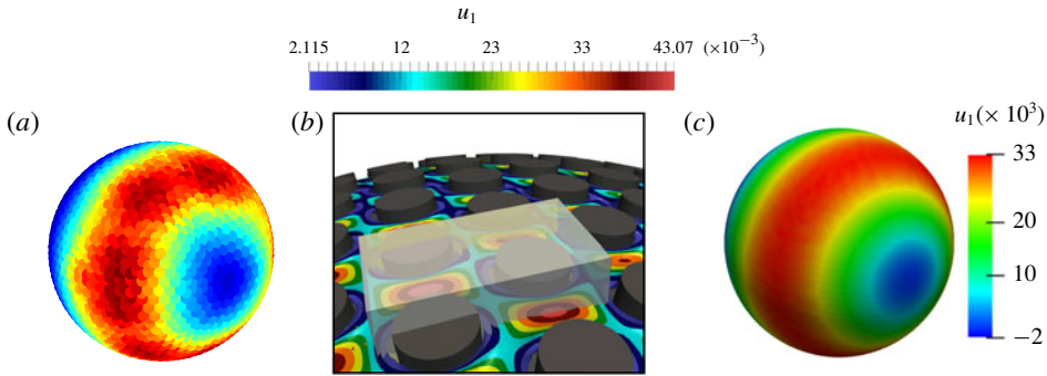
FIGURE 9. (Colour online) Comparison of the streamwise velocity component, u_1 , on the sphere, computed with the macroscopic model (2.28) (c), and extracted from the reference DNS (a). The procedure used to pass from one approach to the other is detailed in the text. (b) The microscopic cell, \mathbb{V} , (in grey), with the microscopic distribution of the u_1 iso-contours on a surface located slightly above R = 1 .
