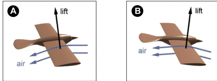
Figure 2.2: In gliding flight, a bird's wing deflects air downward, causing a lift force that holds the bird up in the air (see figure A). By tilting forward and going into a slight dive (figure B), the bird can maintain forward speed.
