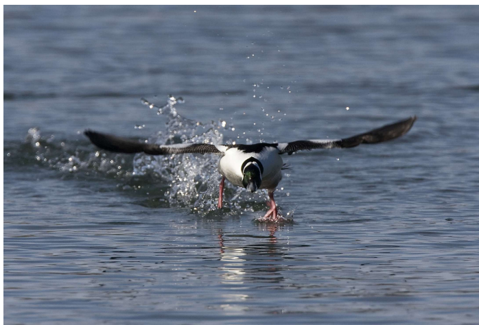
Figure 2.10: A bufflehead running atop the water while taking off.
