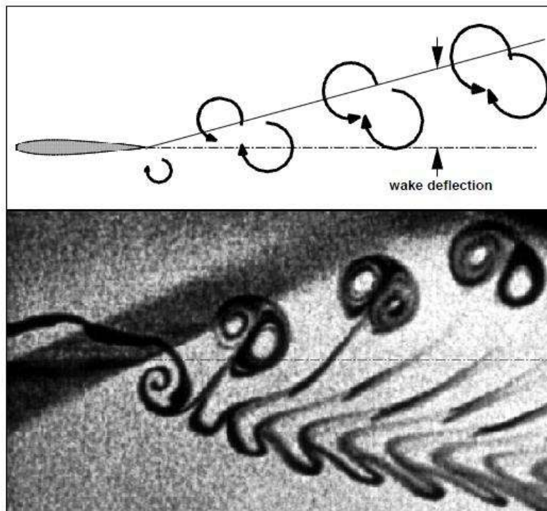
Figure 2.17: Dual-mode or nonsymmetric vortex street indicative of thrust and lift production (deflected wake) [93].
