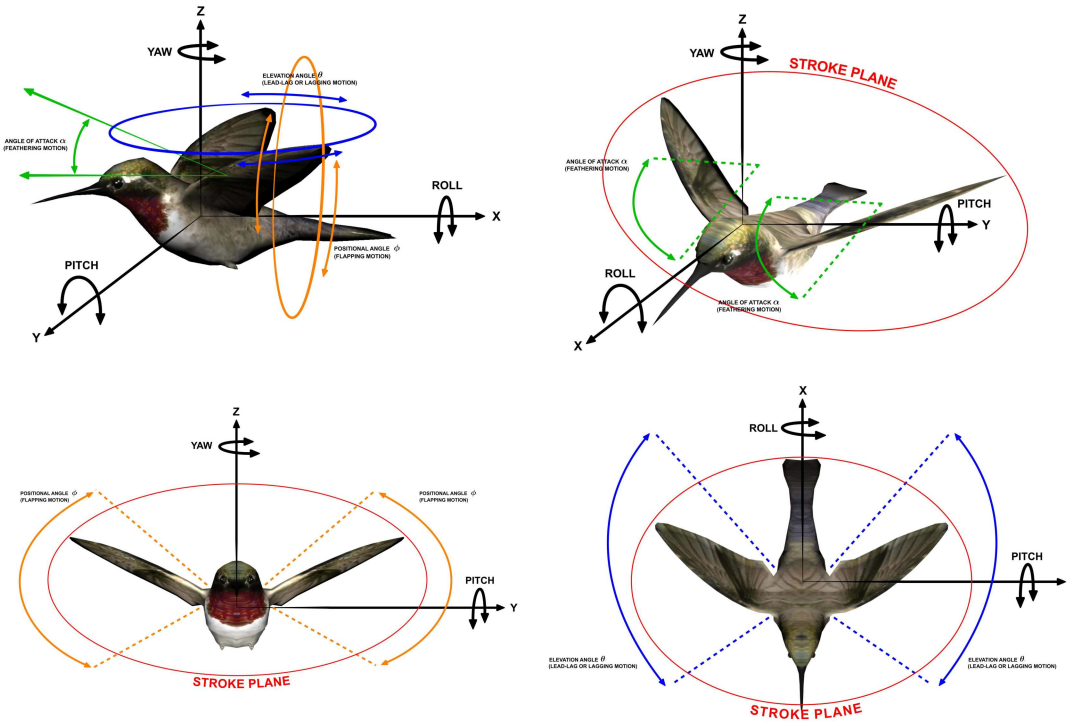
Figure 2.21: 3D flapping wing kinematics.
