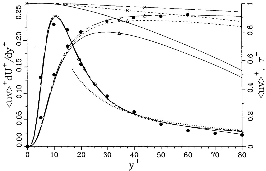
Figure 9. Stresses and production near the wall. — R_\theta = 300 ; - - - R_\theta = 670 ; - · - R_\theta = 1410 . ... 1/\kappa y^+ . \Delta Reynolds stress; \times total stress; \circ production. \bullet Kim et al. 1968.
